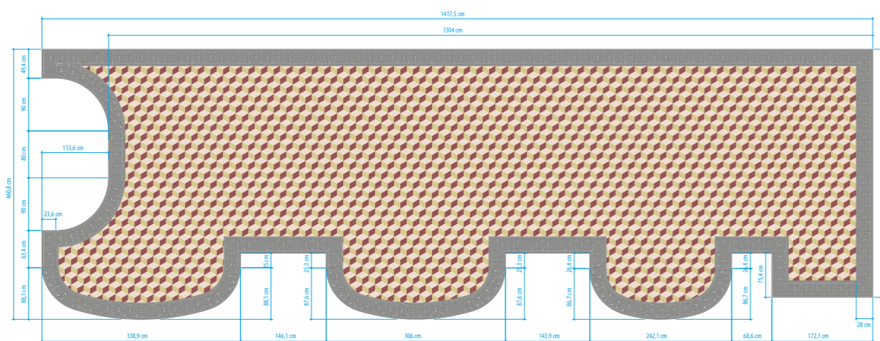
Restaurant Mezzanine Floor Plan · Artistic Marble Mosaic Floor Decor Development
